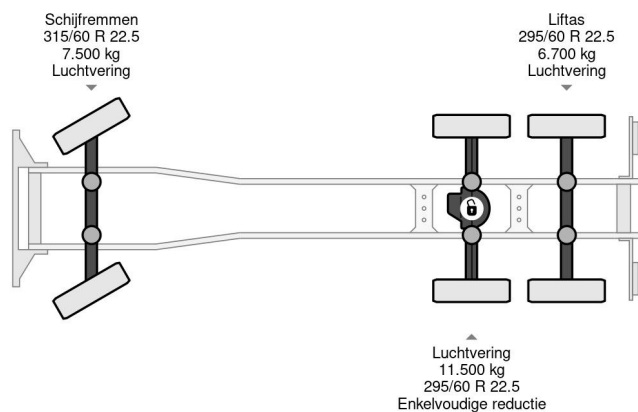
DAF XF 480 SSC 6x2 Volume Combi
