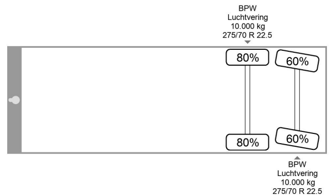
Fruehauf ONCRS 32-220 A | Carrier
