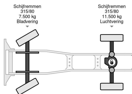
Mercedes-Benz Actros 1845 Retarder | Hydraulic
